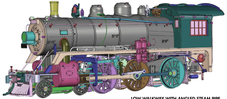
LOW WALKWAY WITH ANGLED STEAM PIPE
