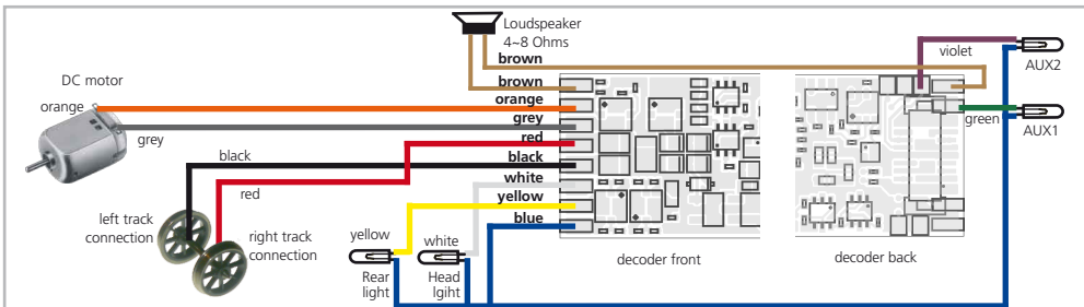
Figure 2: General wiring diagram of LokSound Select micro
